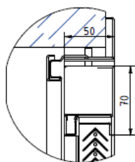
DETAIL B
